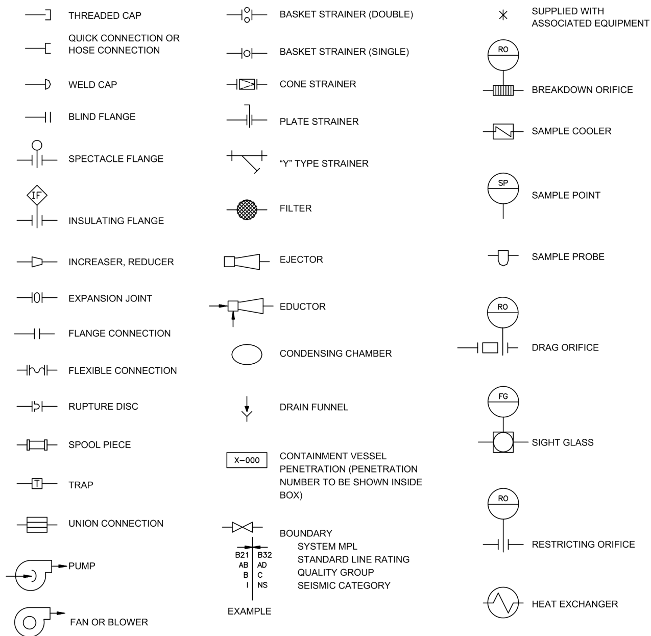
Figure 1.7-3. Miscellaneous P&amp;ID Symbols
