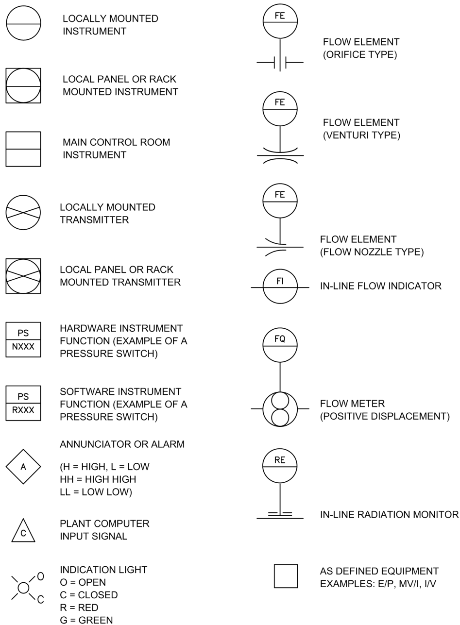
Figure 1.7-2. P&amp;ID Symbols for Instruments
